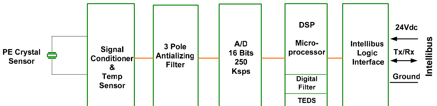
Smart Piezoelectric Accelerometer Functional Diagram
