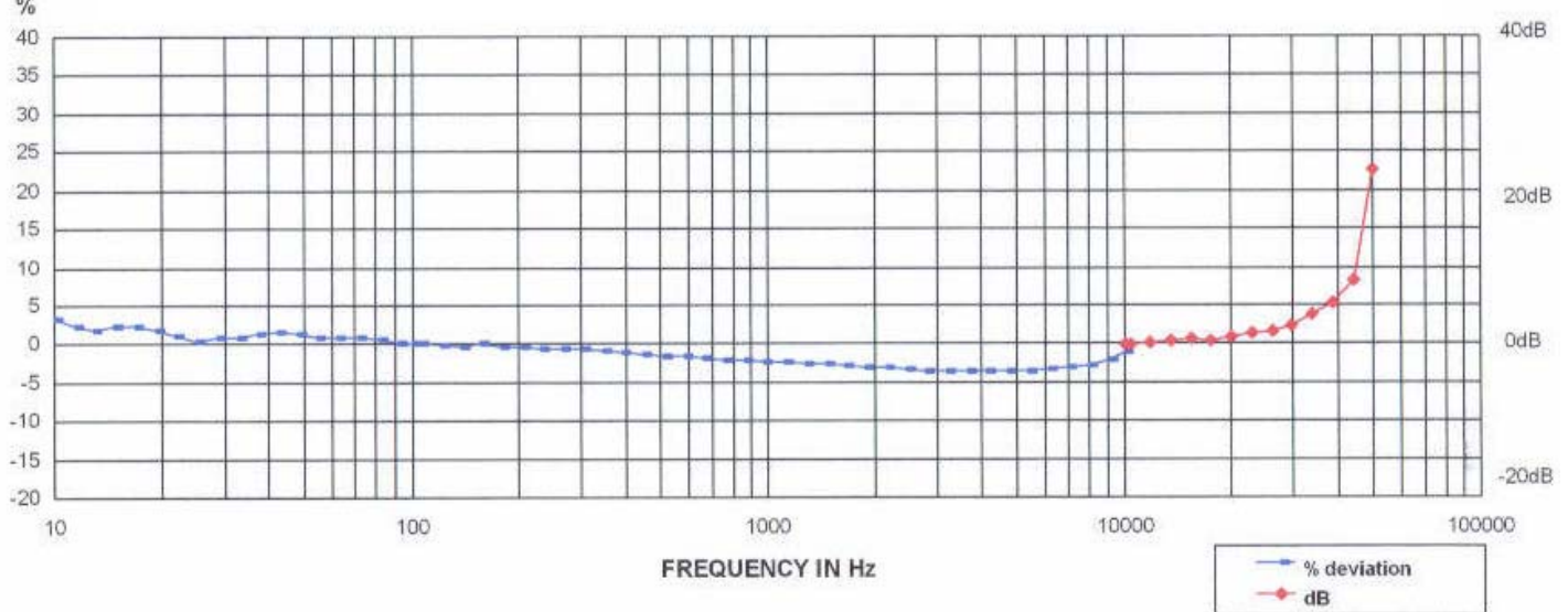
Typical Frequency Response of Accelerometer
